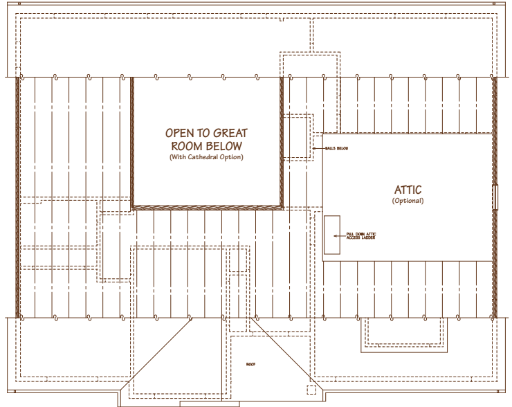
Attic Plan
