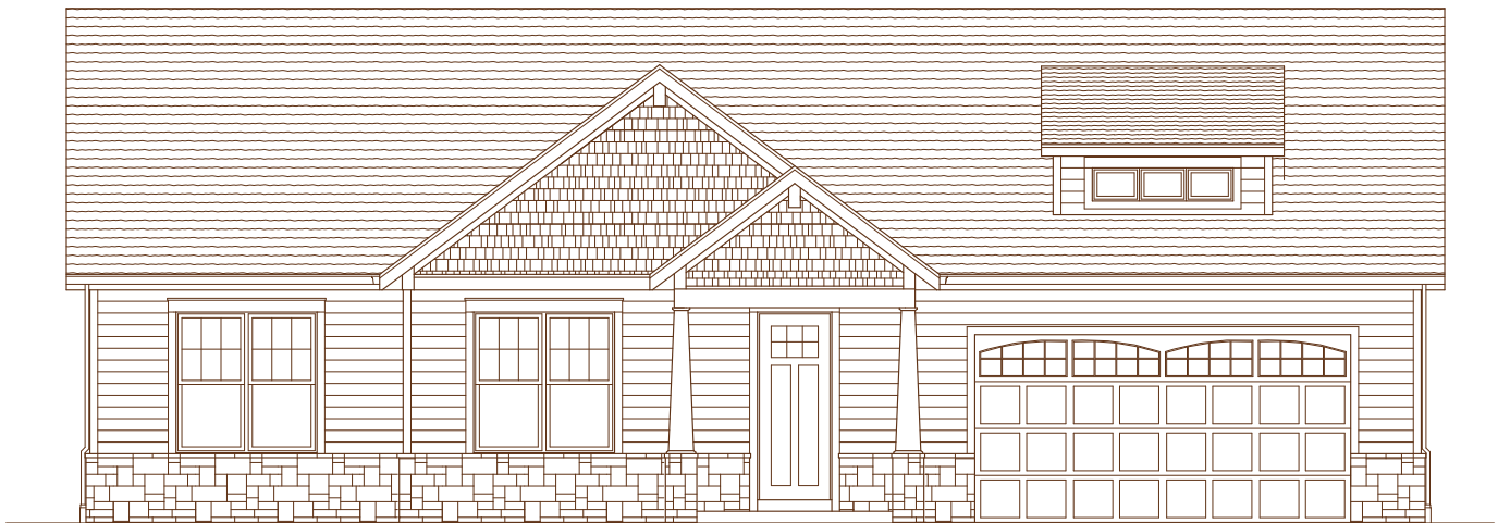
Front Elevation with Optional Porch Extension
