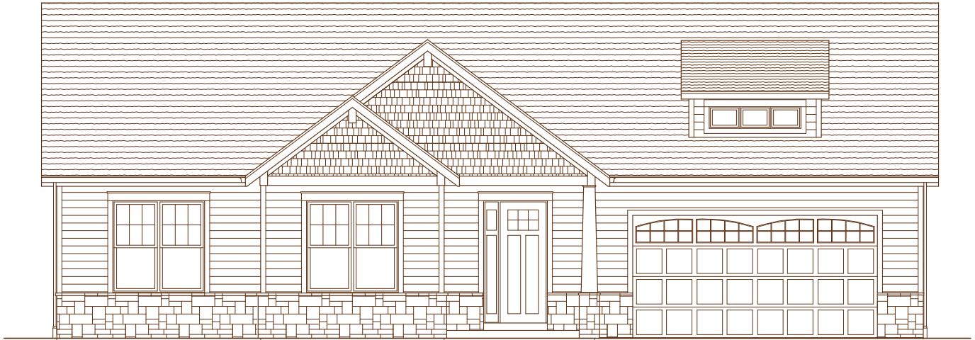
Standard Elevation
