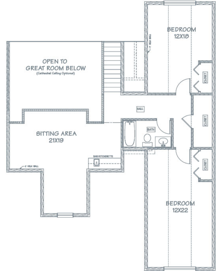
Second Floor Plan (Optional) Approx. 1,000 Livable Sq.Ft.
