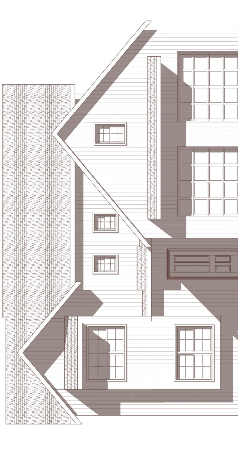
Front Elevation
