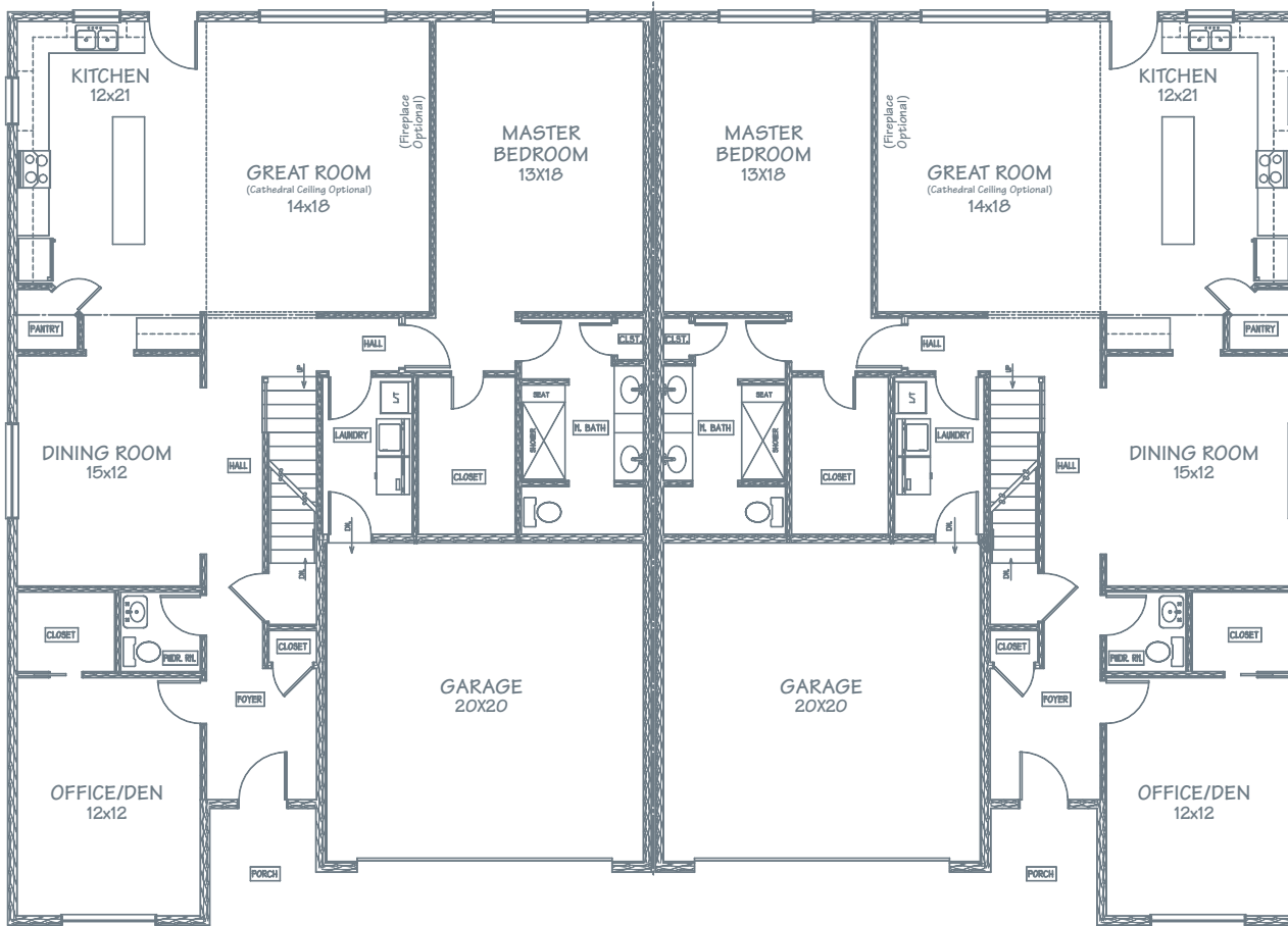
First Floor Plan Approx. 1,840 Livable Sq.Ft.
