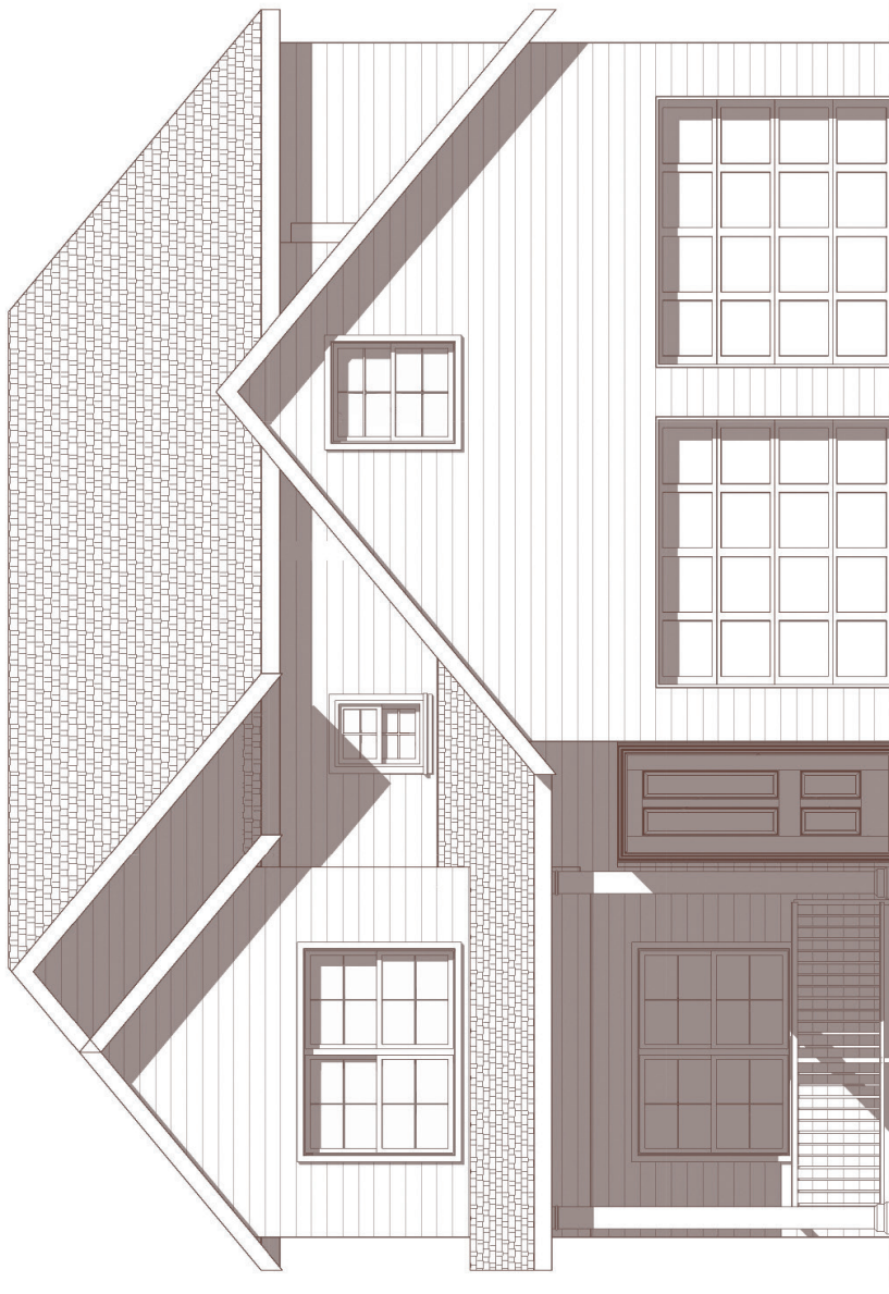
Front Elevation
